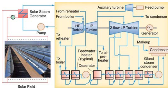
Illustration of a possible steam cycle in which a solar field supplies steam to a pulverized coal plant.
